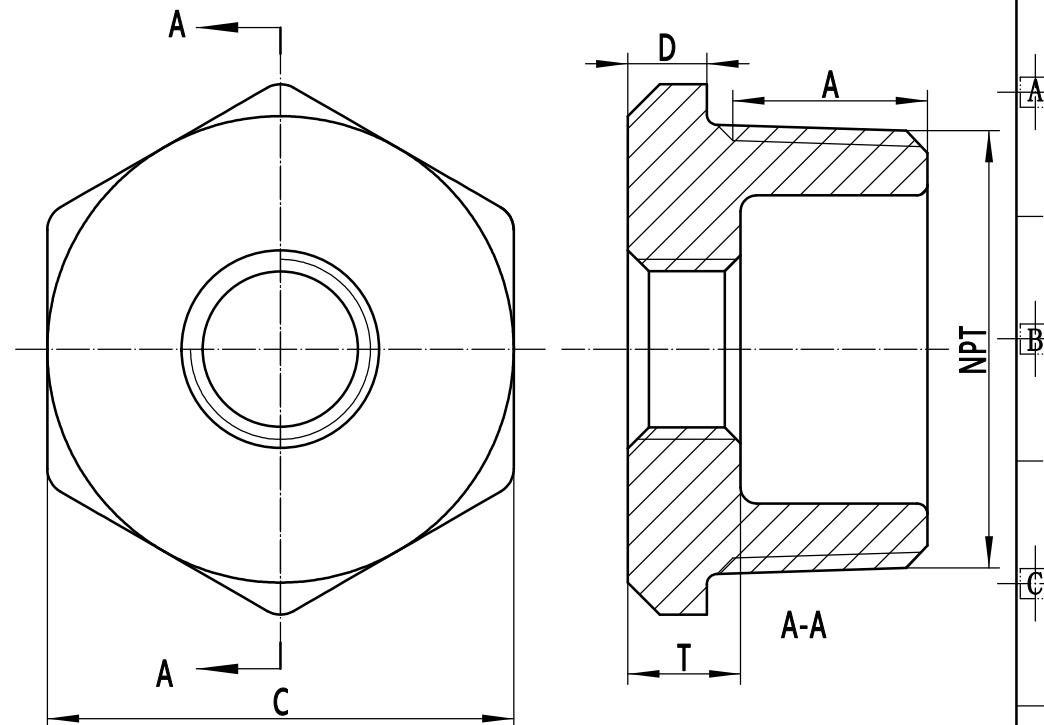
Dimensional Tolerance of Casting (GB/T6414-1999 CT-6)
